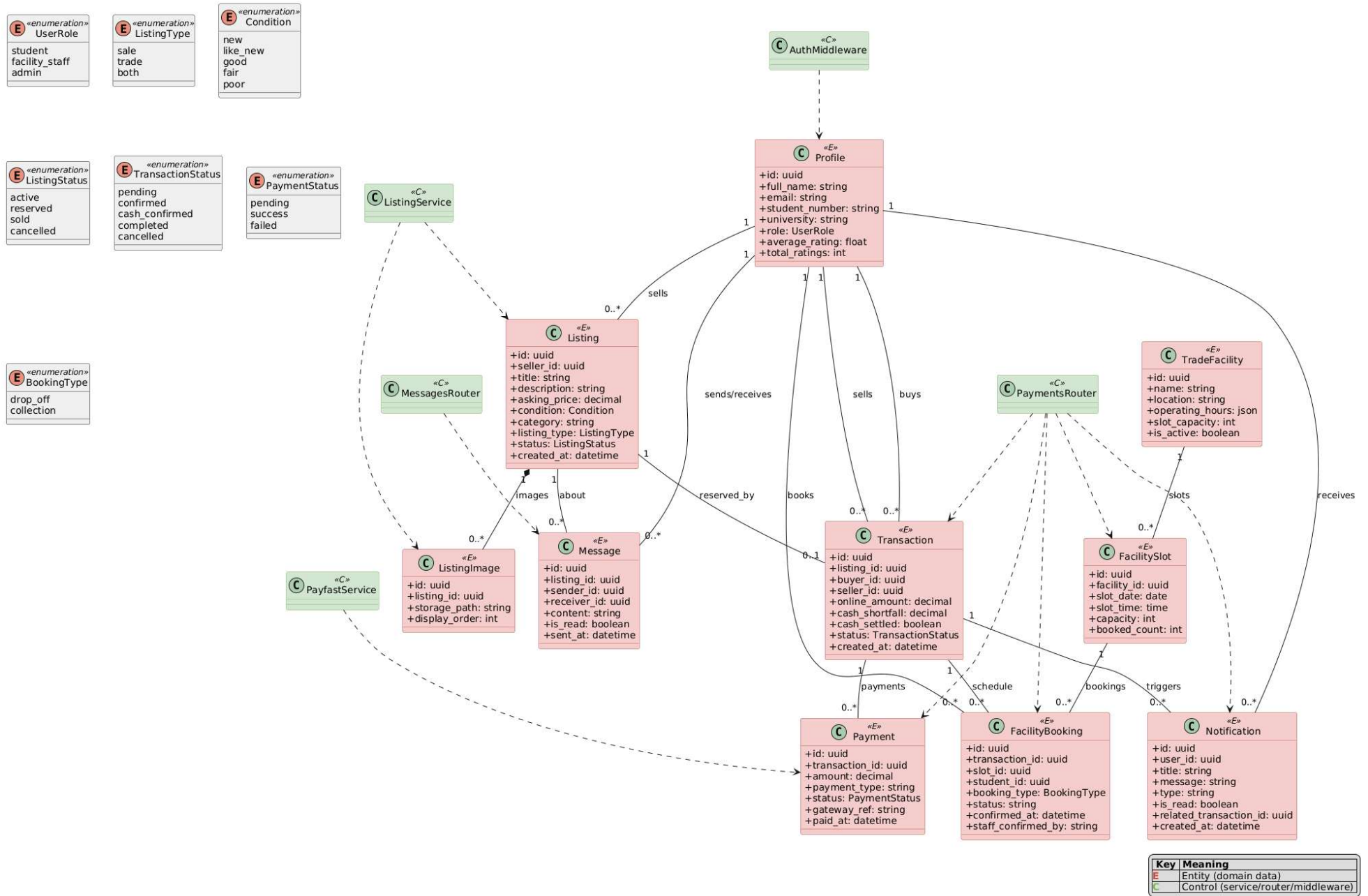
Domain Class Diagram - Marketplace + Payments
